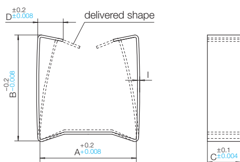
shown Spring-Clip SB-EF 10
