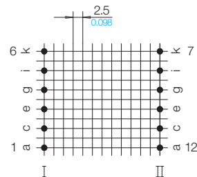
Grid View pin-side
