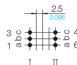
Grid View pin-side
