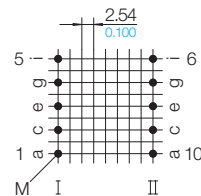
Grid View pin-side
