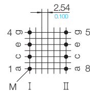
Grid View pin-side
