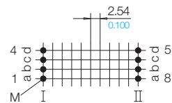
Grid View pin-side
