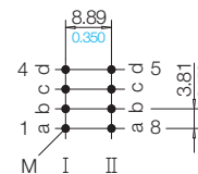
Grid View pin-side
