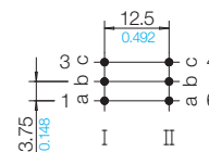
Grid View pin-side
